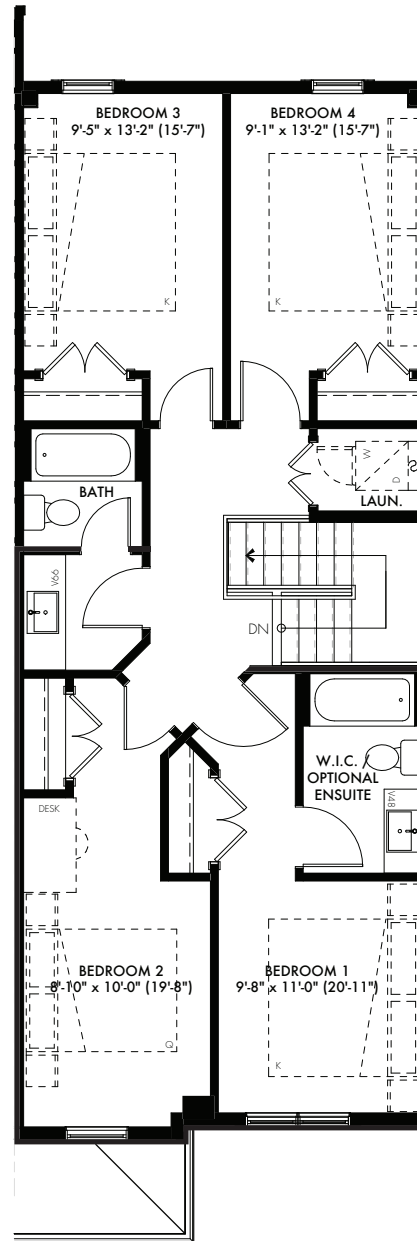
OPT. SECOND FLOOR 937 SQ FT (4 BEDROOM)
