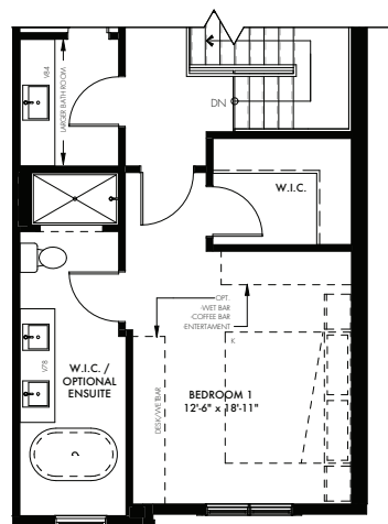
PRIMARY RETREAT OPT. A (3 BEDROOM)
