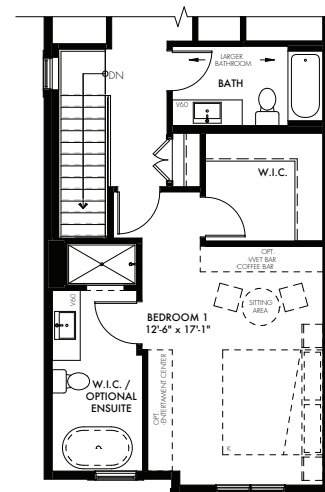
PRIMARY RETREAT OPT. A (3 BEDROOM)
