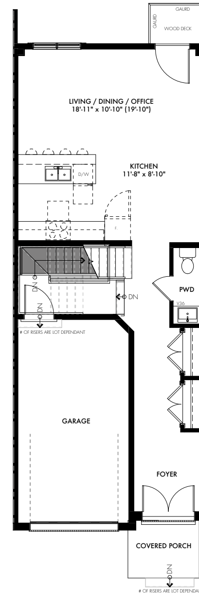
MAIN FLOOR 729 SQ FT
