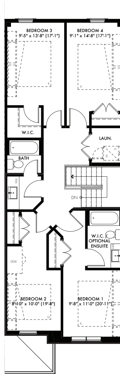
OPT. SECOND FLOOR 999 SQ FT (4 BEDROOM)
