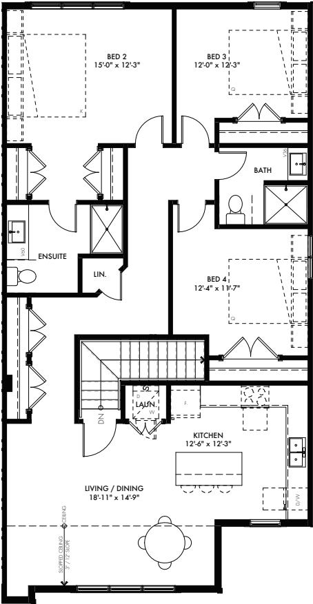
SECOND FLOOR OPT. B
