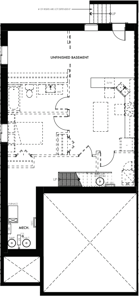
UNFINISHED BASEMENT 991 SQ FT
