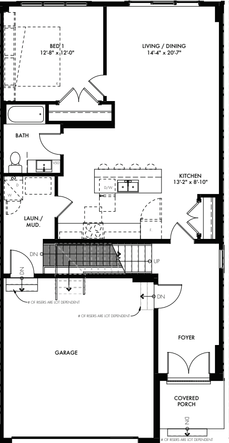
MAIN FLOOR 1106 SQ FT
