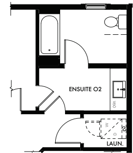
SECOND FLOOR BATHROOM OPT. 2
