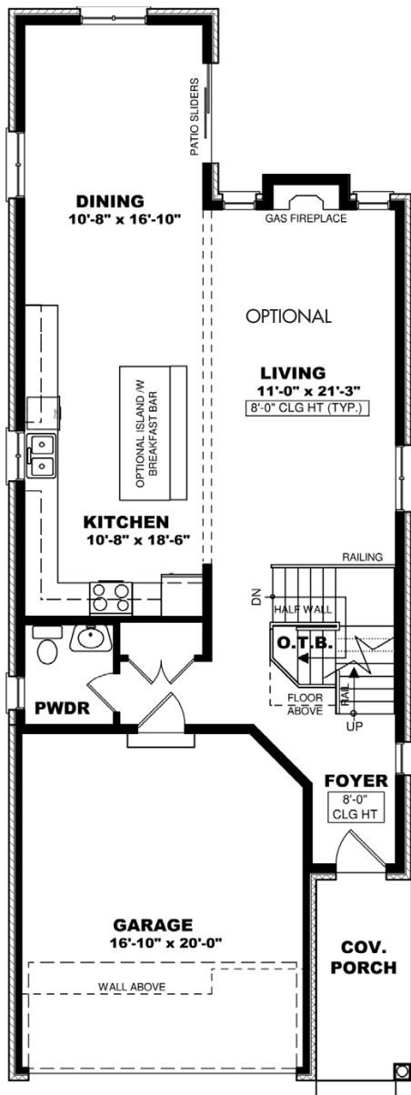
MAIN FLOOR PLAN - 980 SQ FT
