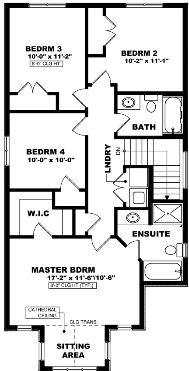
SECOND FLOOR PLAN - 1052 SQ FT
