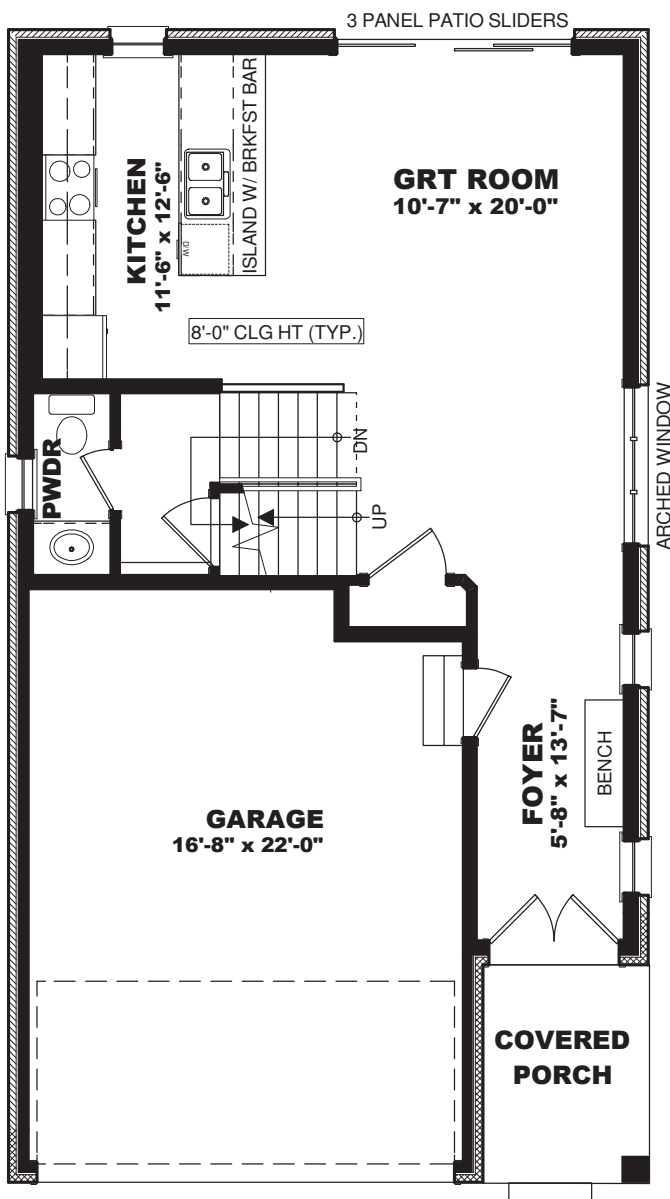
MAIN FLOOR PLAN - 645 SQ FT
