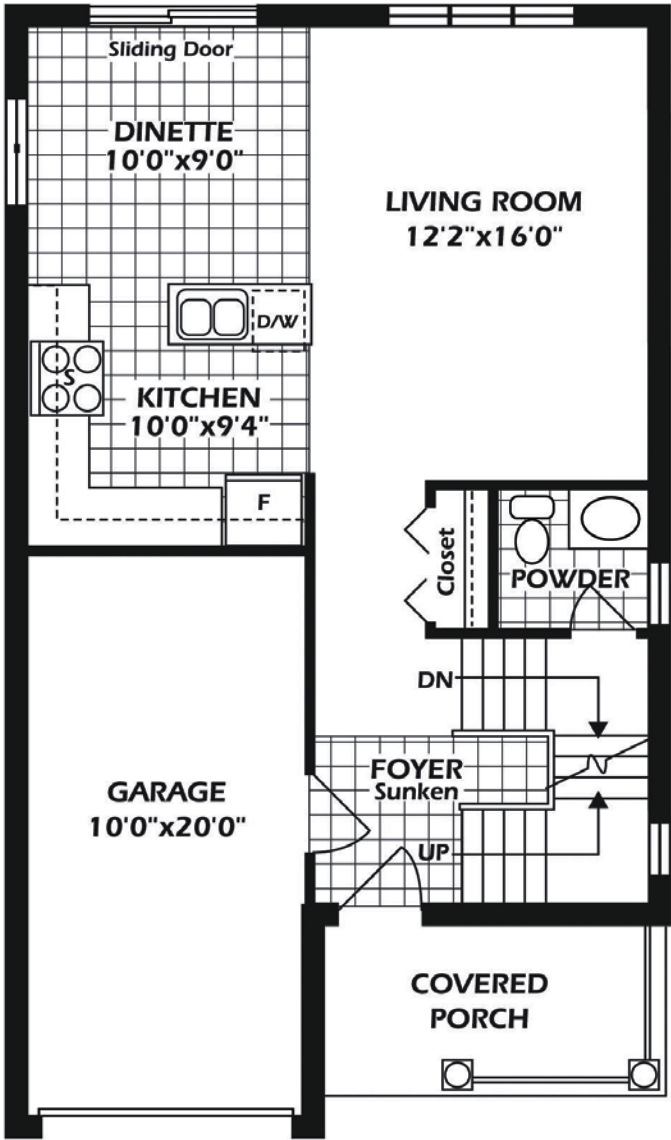
MAIN FLOOR PLAN - 649 SQ FT
