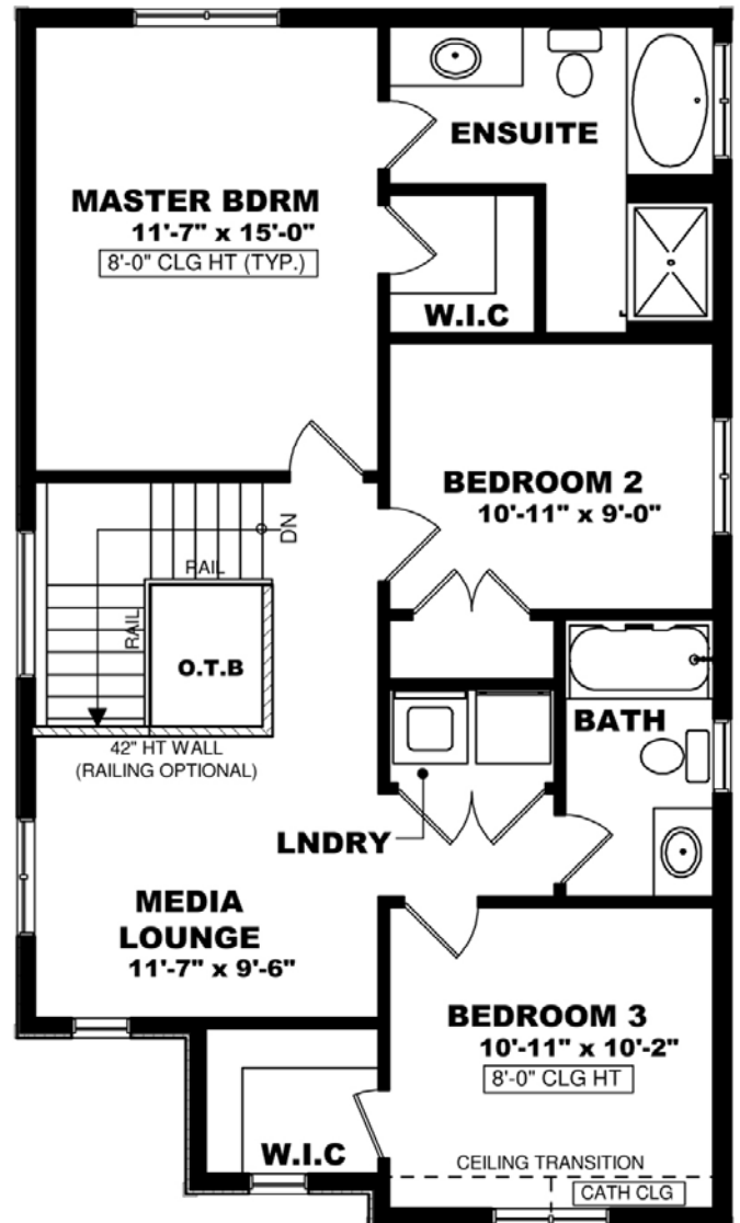
SECOND FLOOR PLAN - 921 SQ FT
