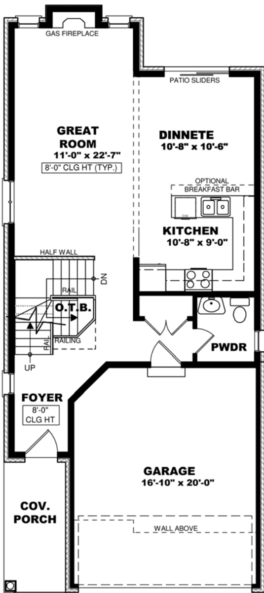
MAIN FLOOR PLAN - 778 SQ FT
