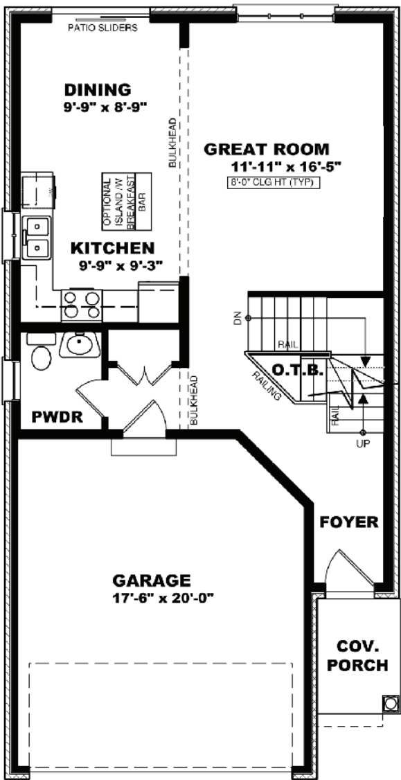
MAIN FLOOR PLAN - 684 SQ FT
