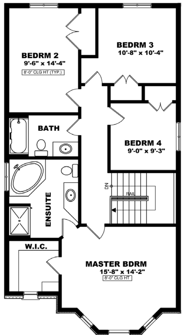
SECOND FLOOR PLAN - 1029 SQ FT
