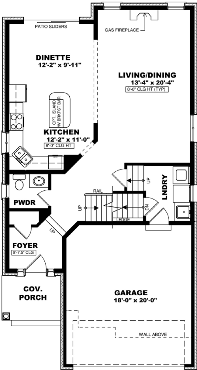
MAIN FLOOR PLAN - 926 SQ FT
