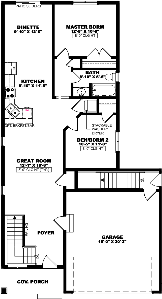
MAIN FLOOR PLAN - 1,096 SQ FT
