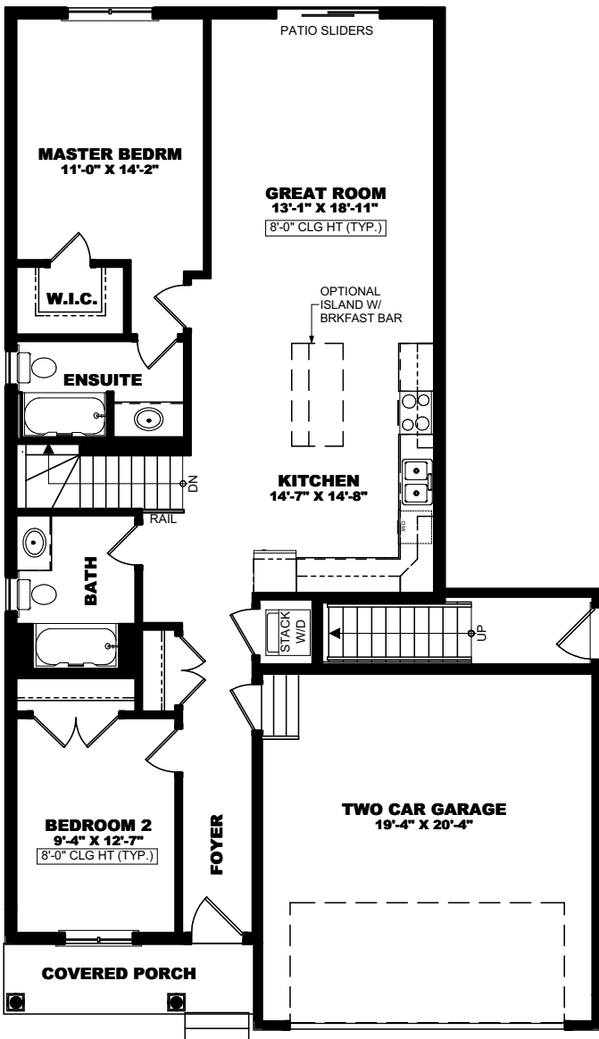
MAIN FLOOR PLAN - 1200 SQ FT
