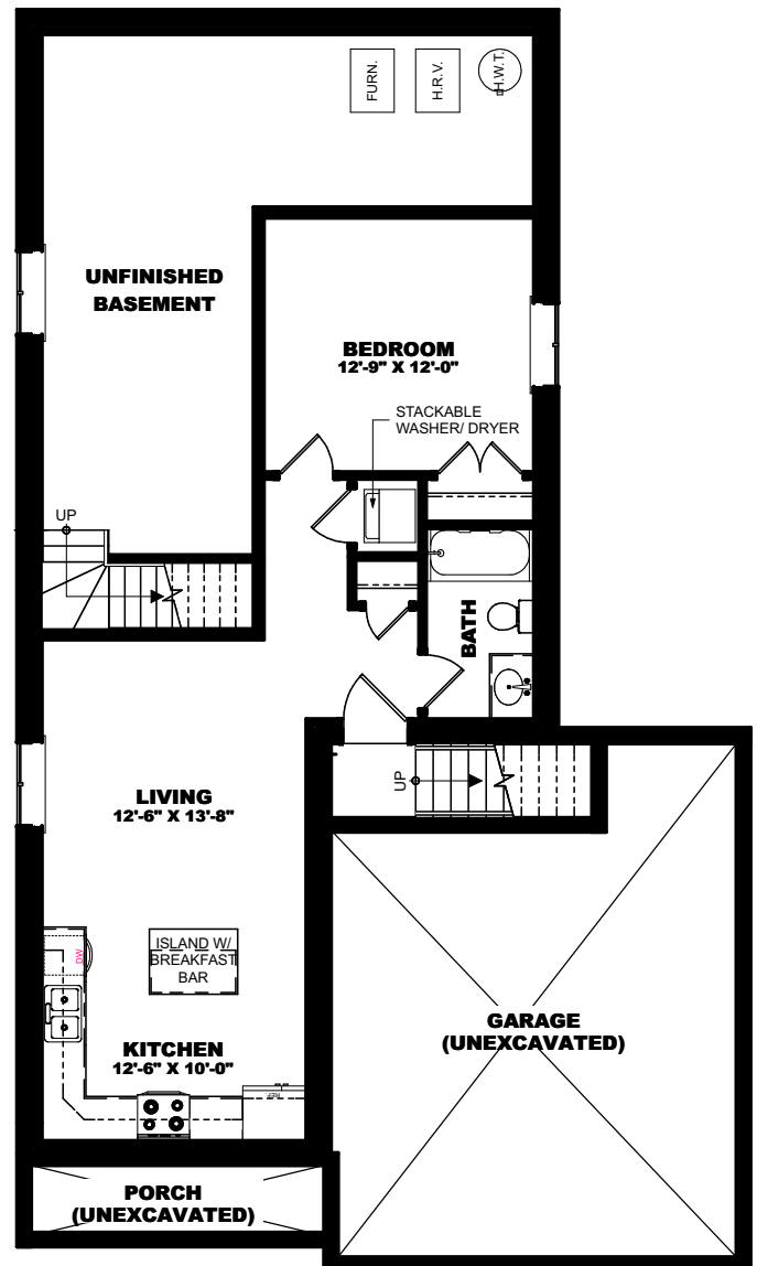
OPTIONAL BASEMENT FLOOR PLAN - 658 SQ FT
