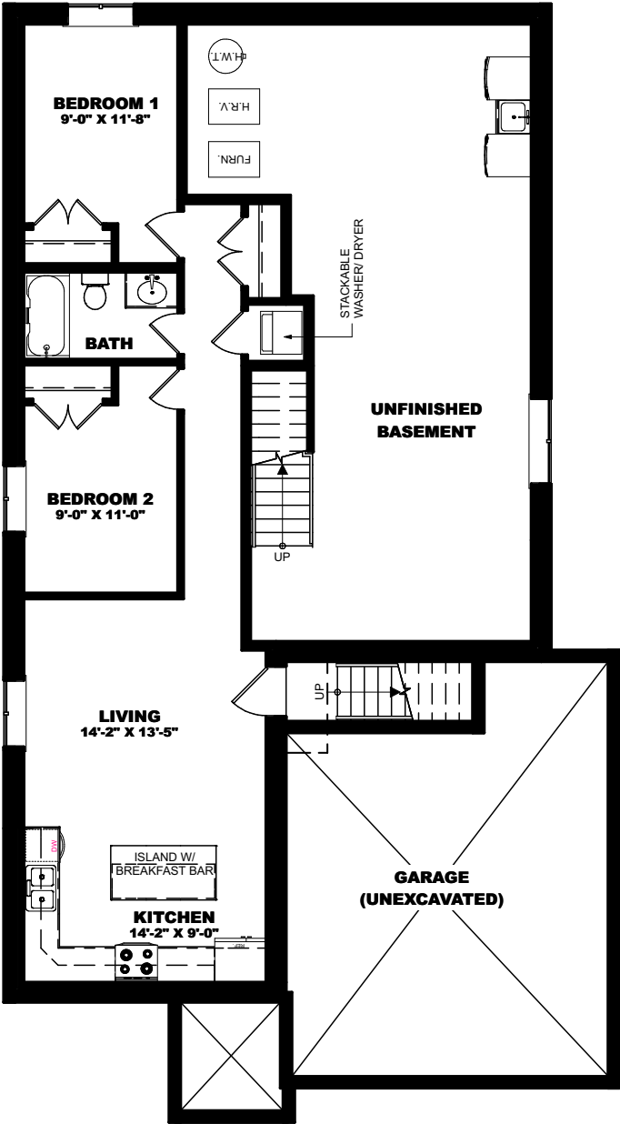
OPTIONAL BASEMENT FLOOR PLAN - 803 SQ FT
