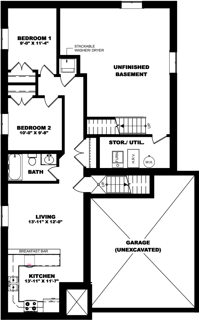
OPTIONAL BASEMENT FLOOR PLAN - 785 SQ FT
