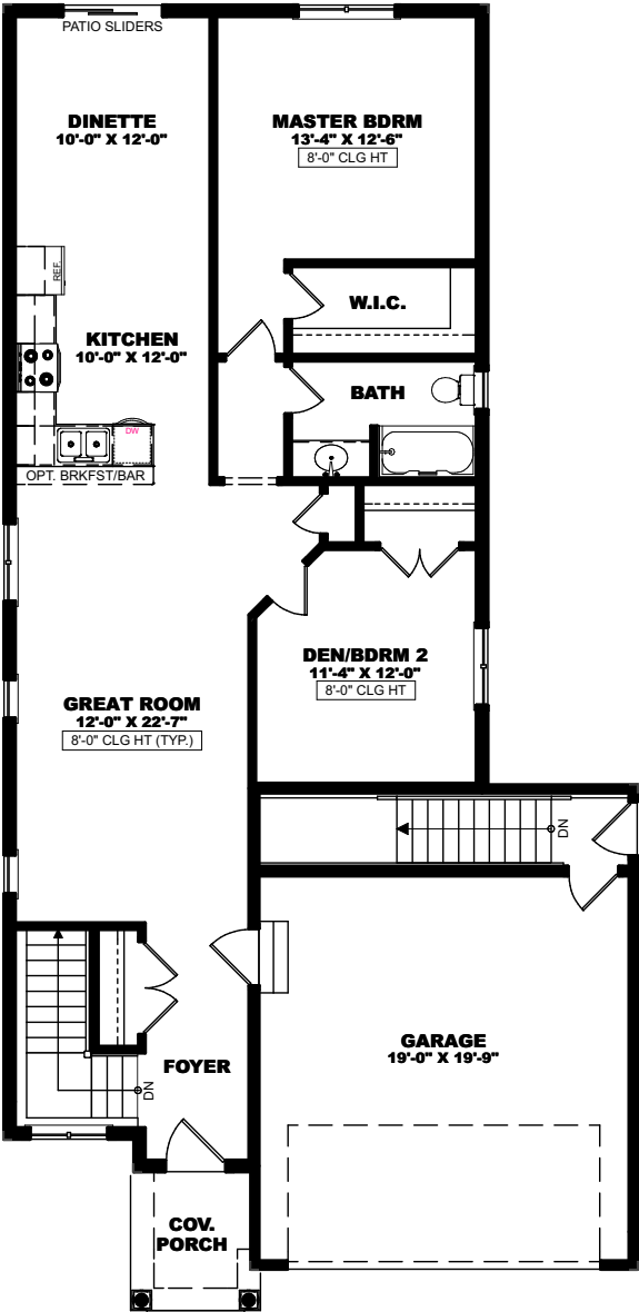
MAIN FLOOR PLAN - 1248 SQ FT
