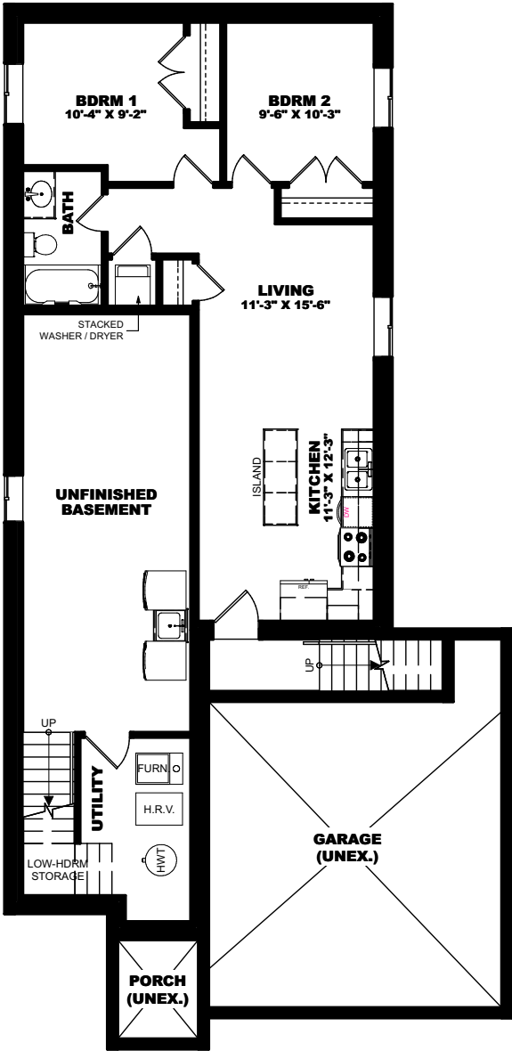
OPTIONAL BASEMENT FLOOR PLAN - 694 SQ FT
