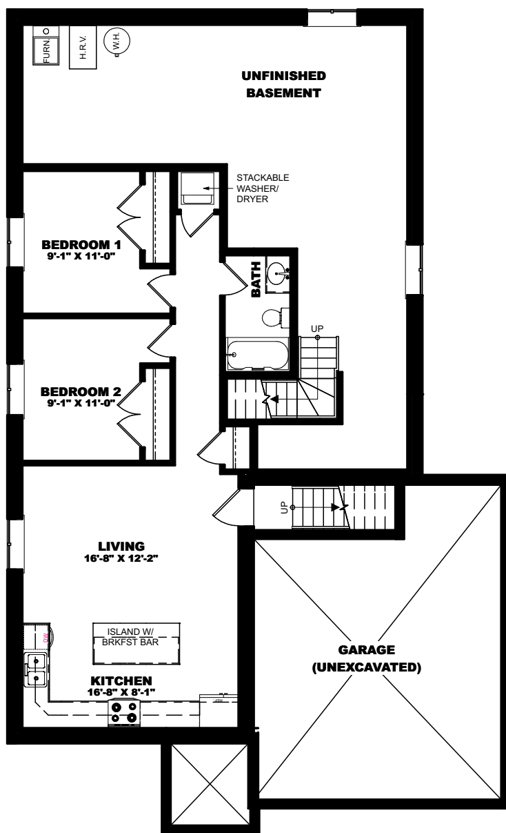
OPTIONAL BASEMENT FLOOR PLAN - 806 SQ FT
