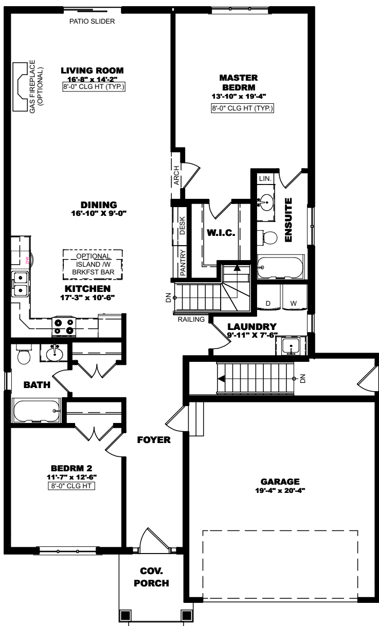
MAIN FLOOR PLAN - 1550 SQ FT
