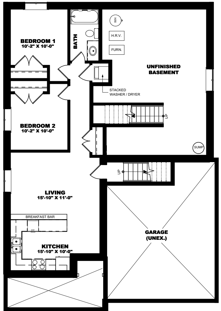
OPTIONAL BASEMENT FLOOR PLAN - 779 SQ FT
