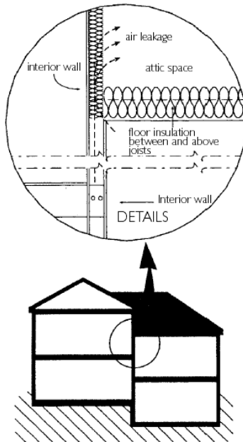
Figure 2: Leakage areas on split level houses
