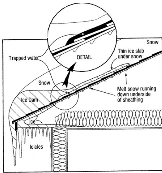
Figure 4: Formation of an ice dam
