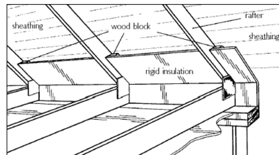
Figure 3: Insulating the outside edge of the attic floor
