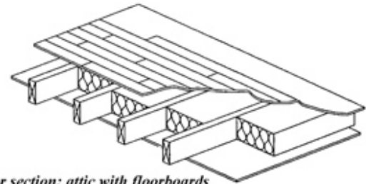
Figure 1: Typical attic floor insulations
